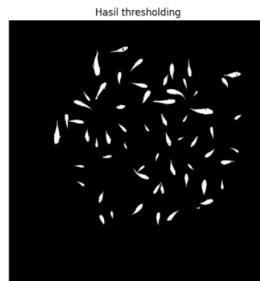
Gambar 5. Hasil Thresholding
