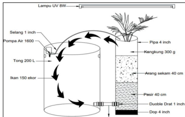
gambar 1. SEQ Gambar \* ARABIC 1. Desain vertiqua biofikal filter
